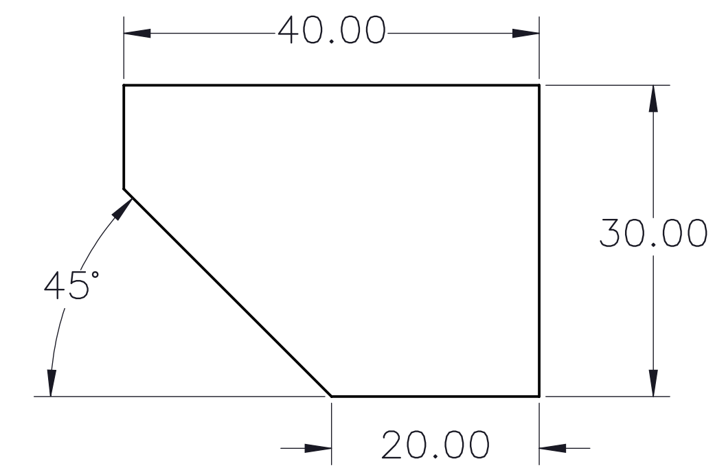
2025-1253-MK01.03-00 HAMMER TAB
