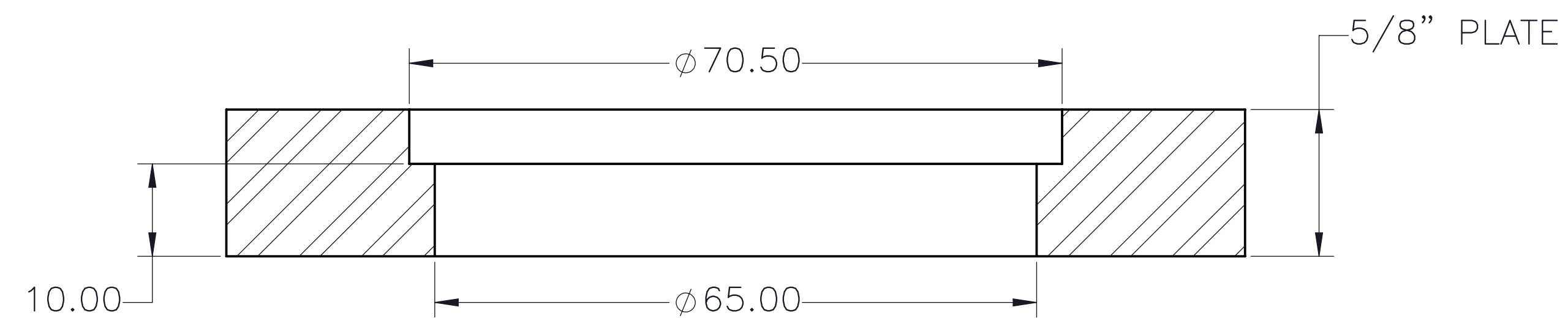
2025-1253-MK01.02-00 LIFTING INSERT FLANGE
